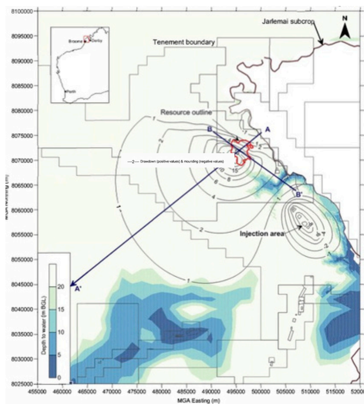
Diagram showing hydrogeological modelling and estimated drawdown profiles
